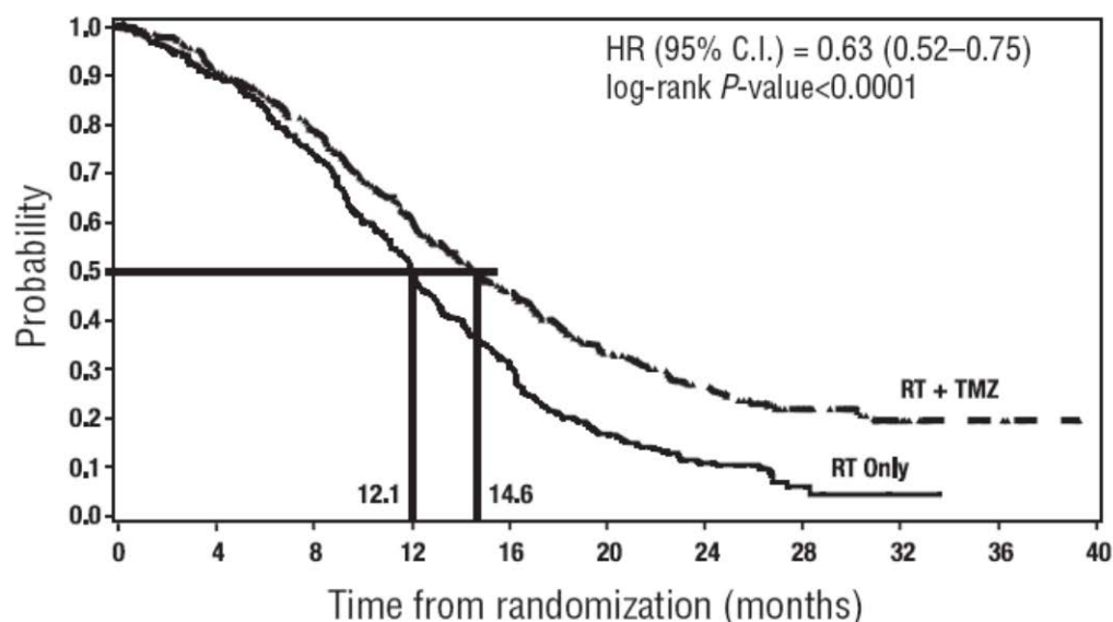
FIGURE 1: Kaplan-Meier Curves for Overall Survival (ITT Population) ITT Population: Overall Survival
